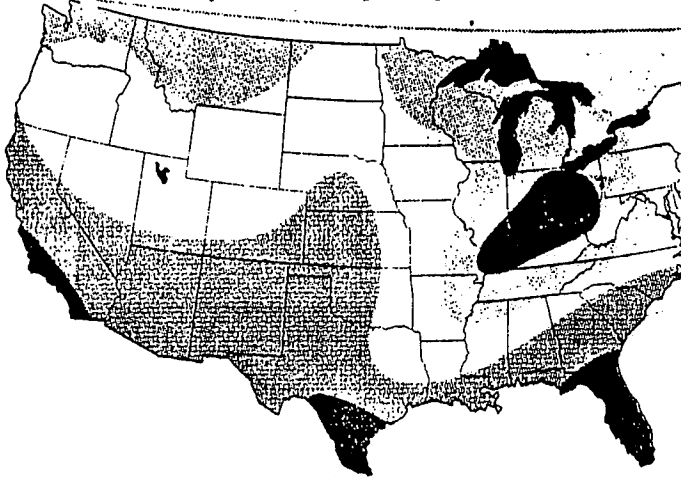
January - March precipitation forecast
